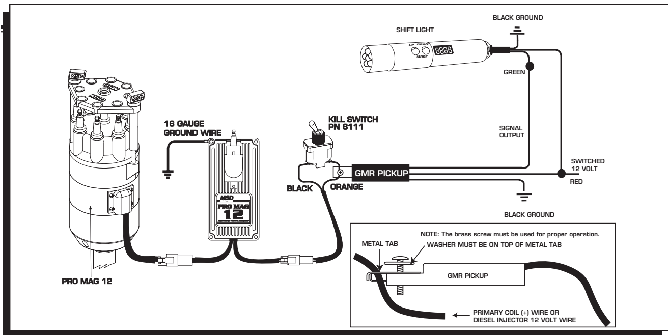
Figure 6 Wiring the 12 Amp Pro Mag.
